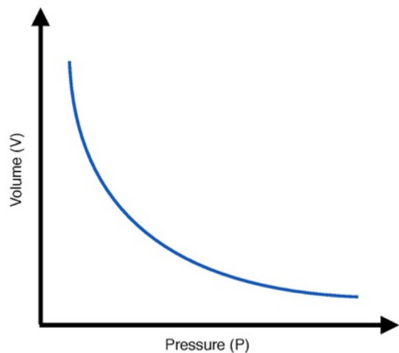
Figure 4: Boyles law
