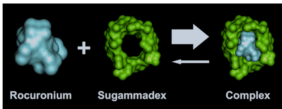
Figure 1: Rocuronium encapsulated by sugammadex. (From Cameron KS, Clark JK, Cooper A, Fielding L, Palin R, Rutherford SJ, Zhang MQ: Modified gamma-cyclodextrins and their rocuronium complexes. Org Lett 2002; 4:3403-6; reproduced with permission)
